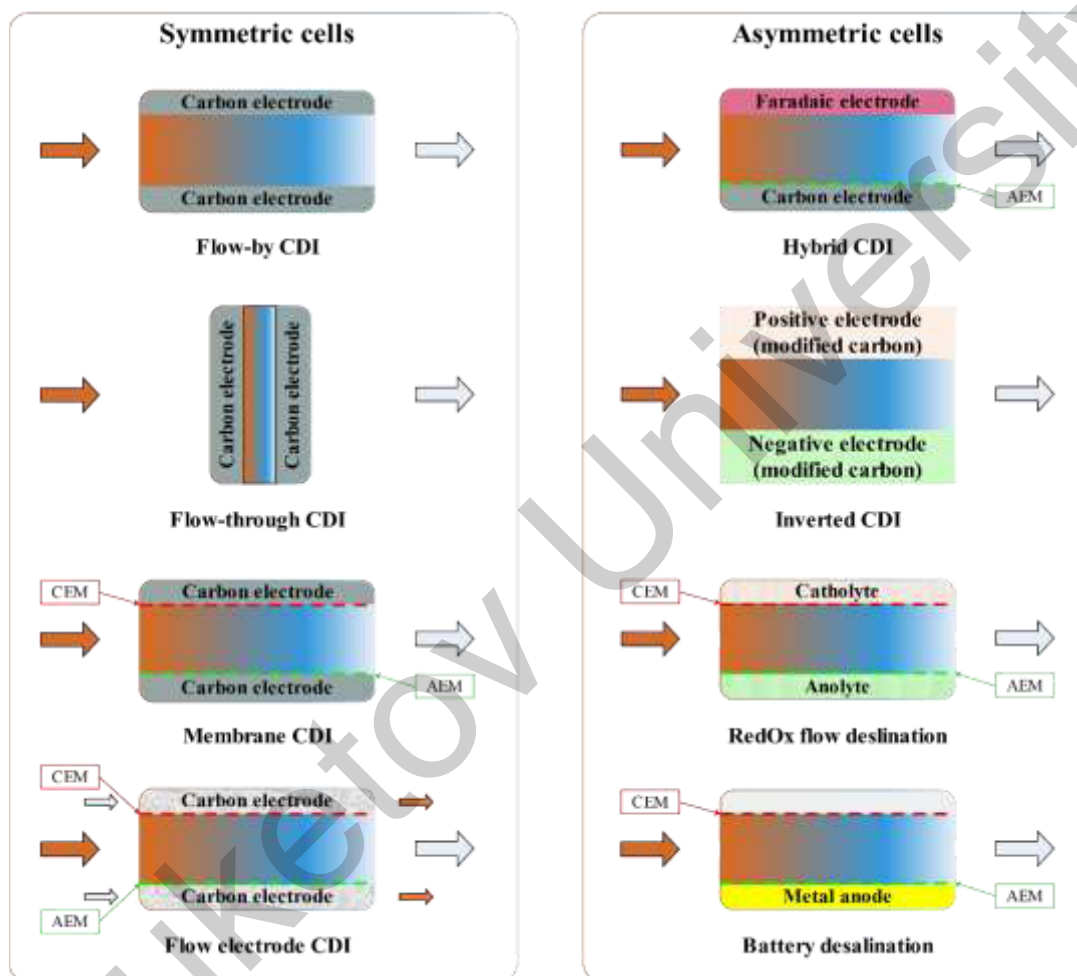
Figure 1. Basic architectures of capacitive deionization cells.
