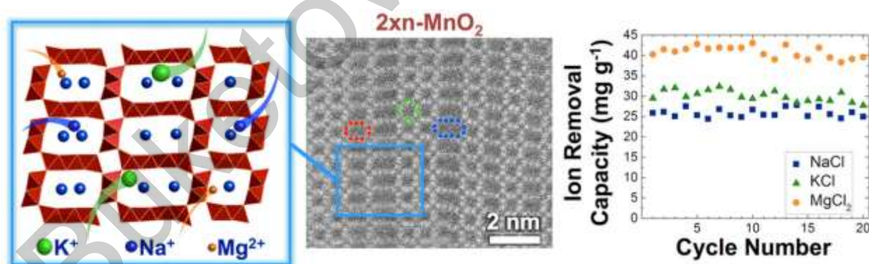
Figure 3. Scheme of available sizes for accumulating ions of various radii in a faradaic material based on MnO 2 structure [103].
