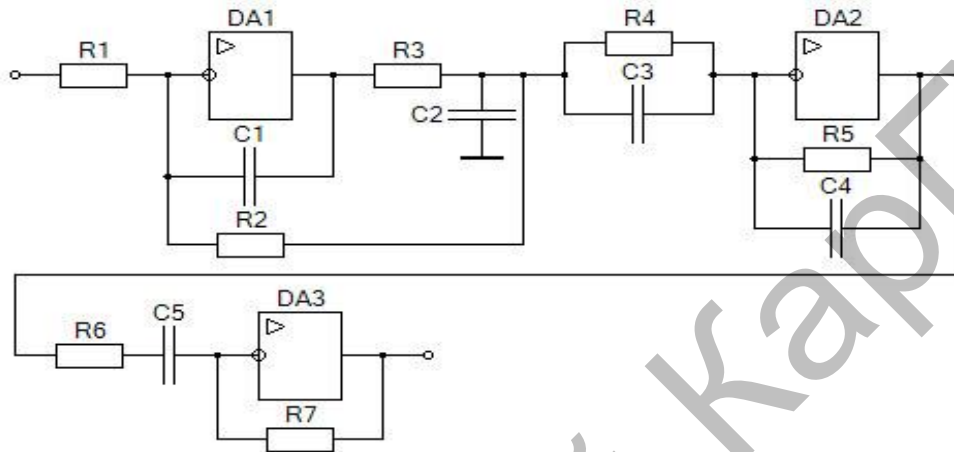
Fig.3. The electrical circuit scheme of filter
