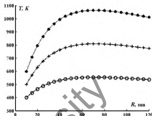
Figure 2. Calculated dependencies of the maximum temperature of the aluminum nanoparticles heated in PETN on its radius at r/R=0.75 and pulse duration 20 ns.
