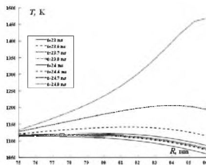
Figure 4. Temperature distributions in PETN surrounding nanoparticle with radius 75 nm (50 nm core and 25 nm shell) at the time moments shown in the legend
