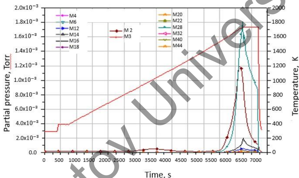
Fig. 4. Gas release from an empty crucible under heating at a speed of 15 K/min
