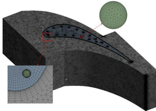
Fig.4. Reference Grid of the Configuration 1 blade.
