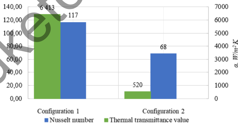
Fig.8. Dependency of the Nusselt Number and the Thermal Transmittance Values on the Topology of the Blade Cooling Baffles.
