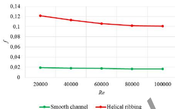
Fig.11. Diagram of Dependency of the Hydraulic Loss Ratio on the Reynolds Number for the Baffles on Review.
