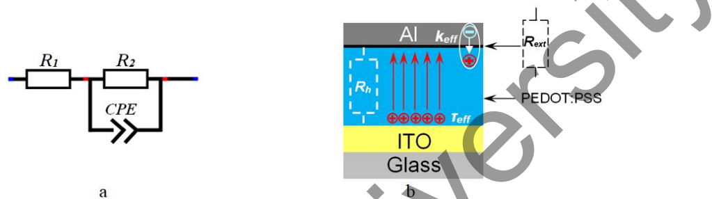
Fig. 4. Equivalent electrical circuit (a) and circuit of charge transport in the cell (b)
