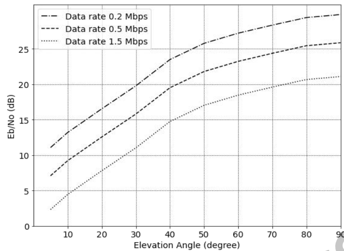
Fig.5. Calculated E_b/N_0 for different data rates for downlink.
