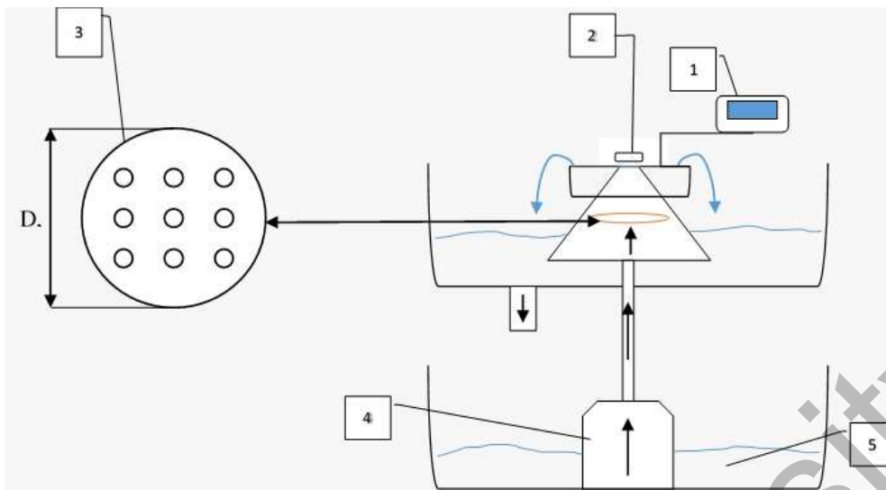
Figure 2. Schematic diagram of an electrolytic cell:
