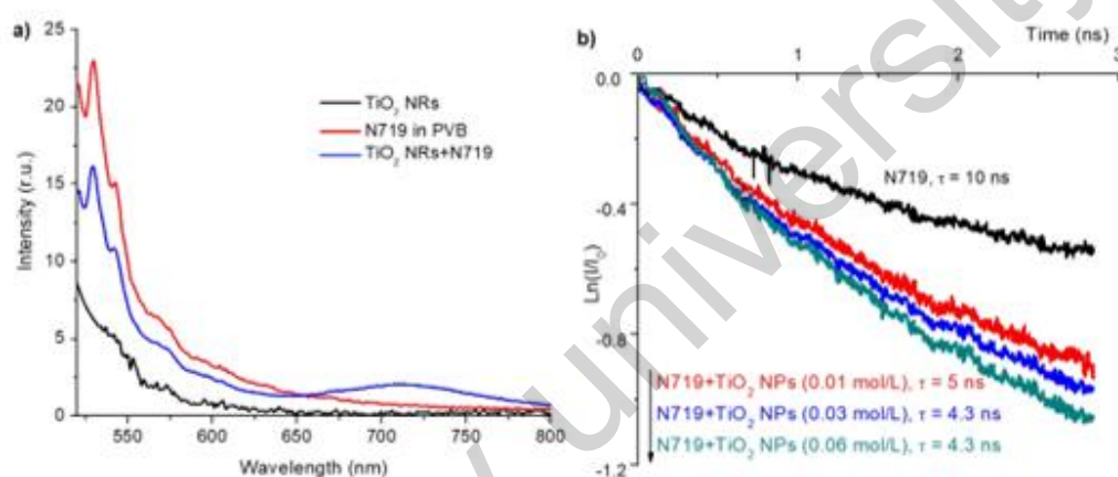
Fig. 5: Fluorescence spectra of N719 molecules in a PVB film and on the surface of TiO 2 NRs doped with dye (a, \lambda_{exc} =510 nm); the influence of concentration of TiO 2 NPs on the fluorescence decay kinetics of N719 dye in PVB film (b, \lambda_{reg} =550 nm).
