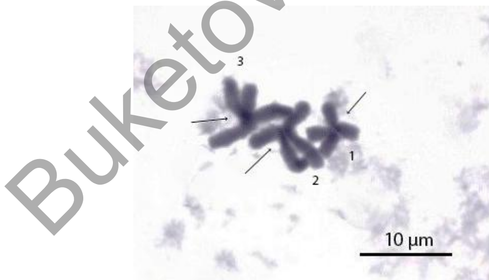
Figure 2. C-stained chromosomes in Ae.cataphylla .
