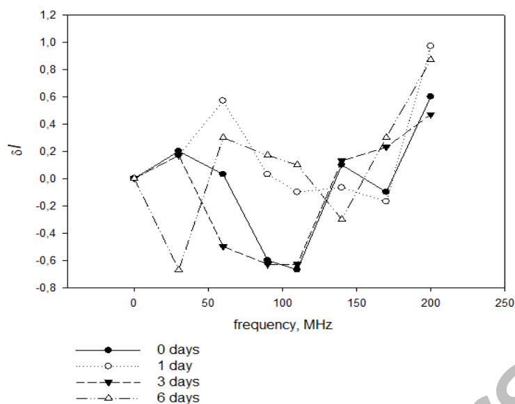
Figure 4. Dependence of the relative change in the length of ice core on the frequency of field effect for different exposure times
