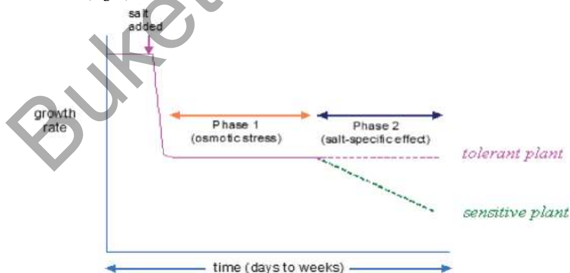
Figure 1. Scheme of the two-phase growth response to salinity [53]
