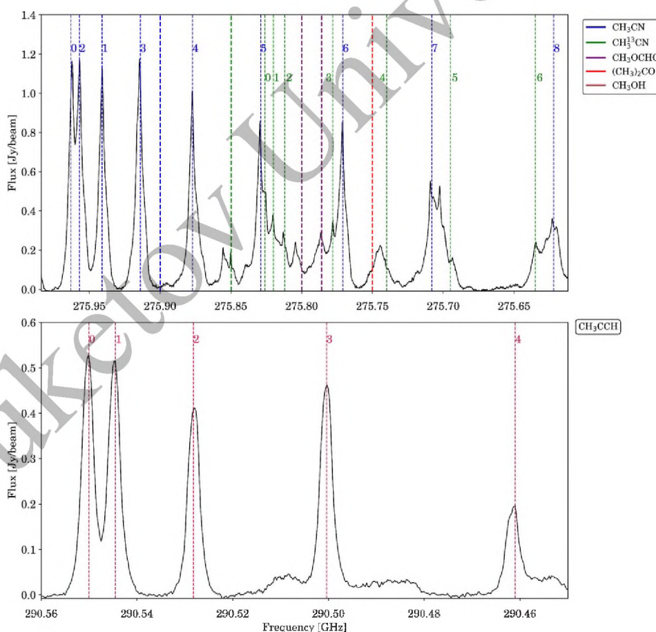
Fig. 2. Molecular line spectra toward G335.79+0.17 P1, extracted from a circular region with a diameter of 0.9'' centered at (\text{RA}, \text{Dec}) = (16:29:47.3388, -48^\circ 15' 52.3963'') .
