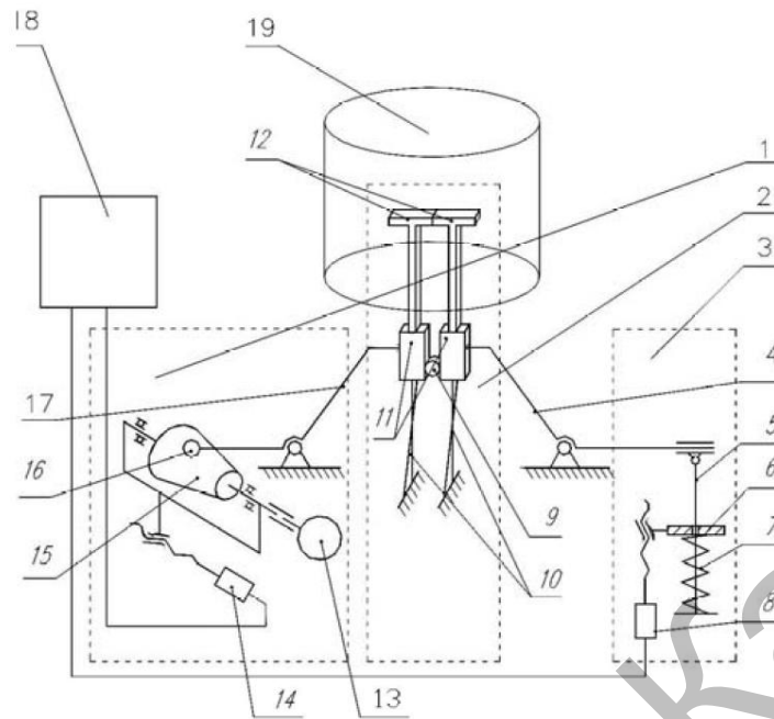
Fig.7. The scheme of the wear analog modeling: 1 –the longitudinal oscillation amplitude setting unit; 2 –samples attachment unit; 3 –load setting unit; 4 –lever; 5 –thrust rod; 6 – thrust washer; 7 – load spring; 8 – stepper motor; 9 – roller; 10 – spring plate clips; 11 – struts; 12 – samples; 13 – electric motor; 14 – stepper motor; 15 – cam; 16 – roller; 17 –tappet arm; 18 – electronic unit; 19 –temperature setting unit chamber.
