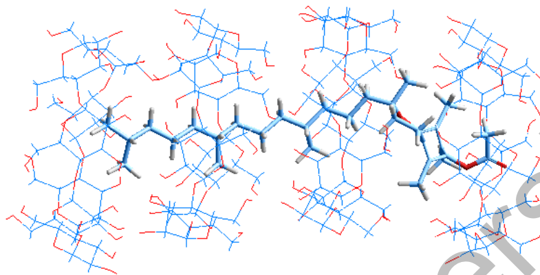
Figure 4. Molecular model of the “ \beta -CD:VE” complex in a ratio of 1:4 ( E_{\text{total}} = -1629877 kcal/mol)
