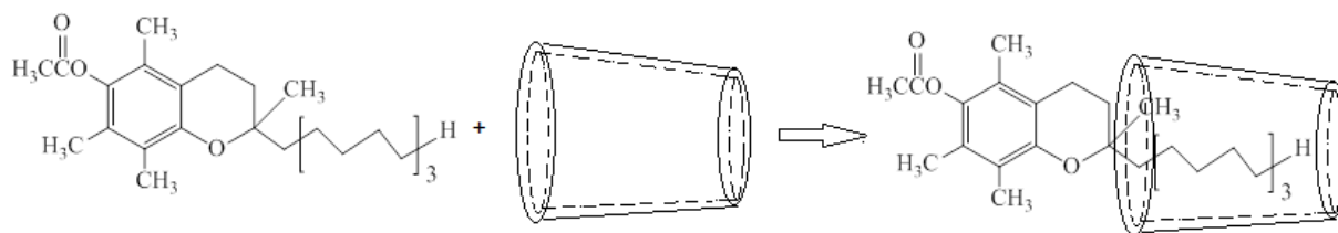
Figure 7. Scheme of the “ \beta -CD:VE” complex formation
