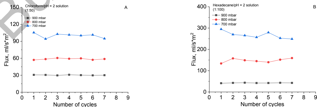
Figure 4. The fluxes of modified PET TeMs-PAAm with pore density 1 \cdot 10^6 for chloroform/pH=2 solution (1:50) and hexadecane/pH=2 solution (1:100) oil-water emulsions after each cycle at different pressure
