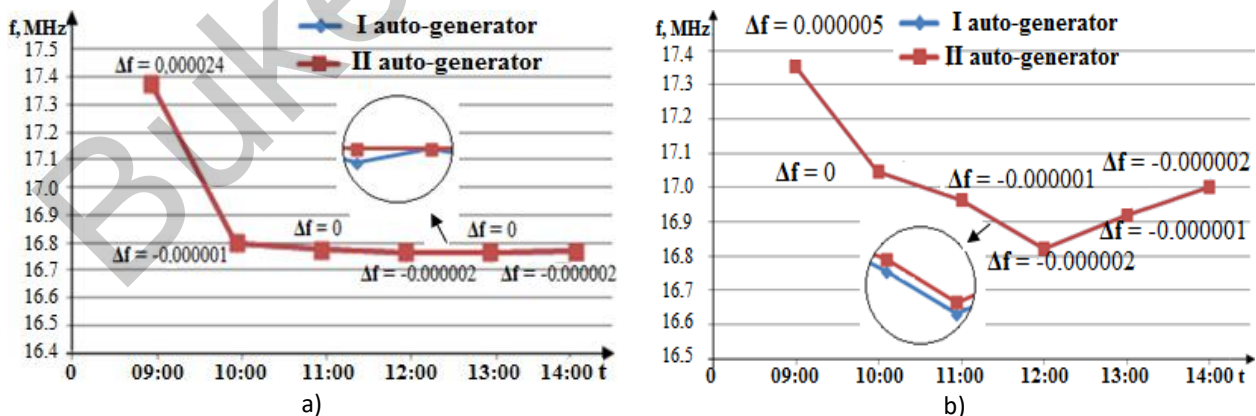
Fig. 3. Frequency variations of auto-generators:
