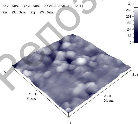
Fig.6. AFM image of the coating Mn-Fe-Cu-Al
