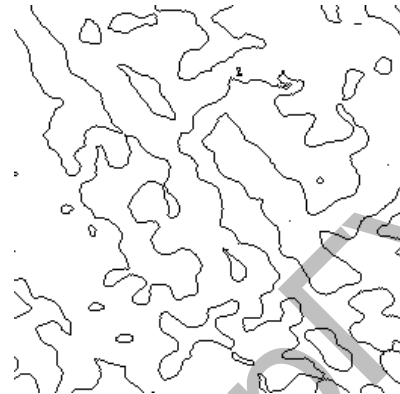
Fig.3. Fractal structure of the Cr-Mn-Si-Cu-Fe-Al+Ti coating
