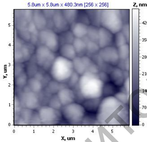
Fig.4. AFM image of the coating Zn-Al
