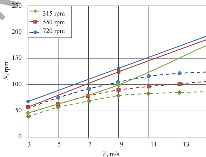
Fig. 4. The dependence of the rotation speed of the wind wheel on the velocity of the incoming flow obtained by the sliding grid method
