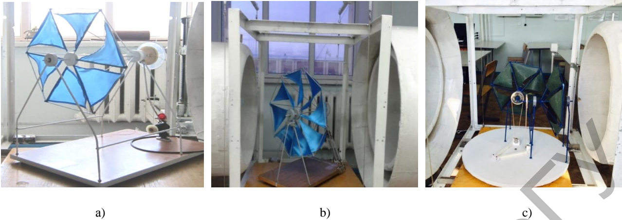
Fig. 1. Models in wind tunnel T-M-1 working section: a) model with six sail blades; b) model with eight sail blades; c) twinned (coupled) combined model with two wind wheels.
