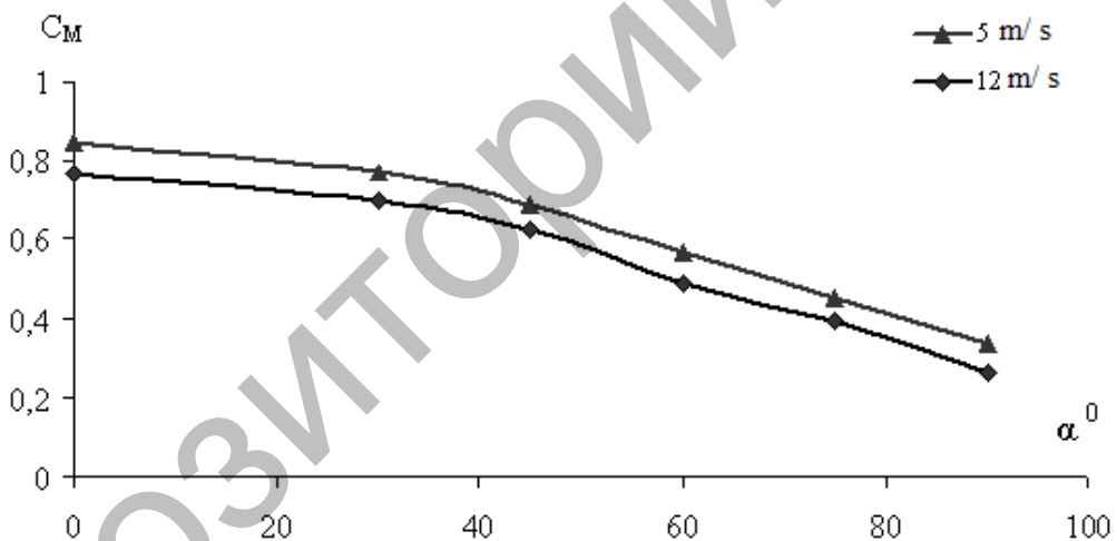
Fig. 5. Dependences of the thrust coefficient of WT-3 wind turbine on the attack angle of the wind flow.
