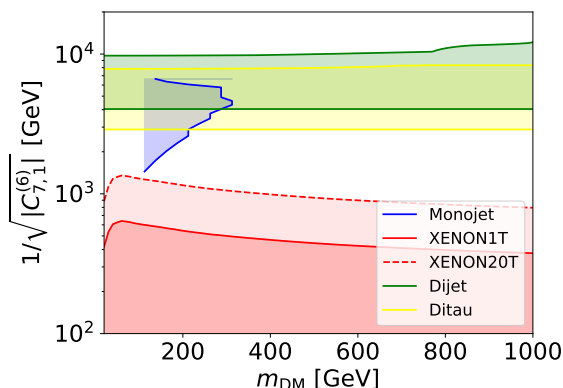
Figure 4. Exclusion limits for the model of table 1 from XENON experiment for 1 ton \times year exposure (red solid) and for 20 ton \times year exposure (red dashed), from LHC monojet (blue) and dijet (green) analyses with 139 \text{ fb}^{-1} integrated luminosity and ditau (yellow) analyses with 19.5\text{--}20.3 \text{ fb}^{-1} integrated luminosity. The results are shown in the plane with the DM mass on the x axis and the inverse of the square root of the Wilson coefficient |C_{7,1}^{(6)}| on the y axis.
