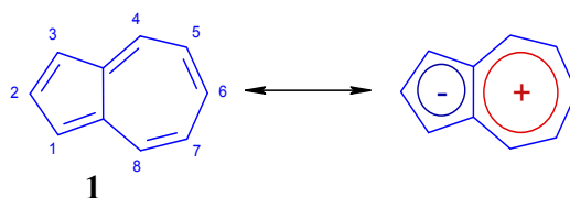
Figure 1. The polarized resonance structure of azulene 1
