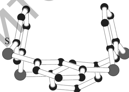
Figure II-25. Structure SAXJEG [10]
