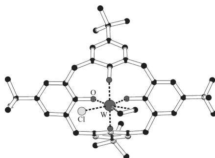
Figure II-2. Structure of tungsten complex GUBTAY [10]
