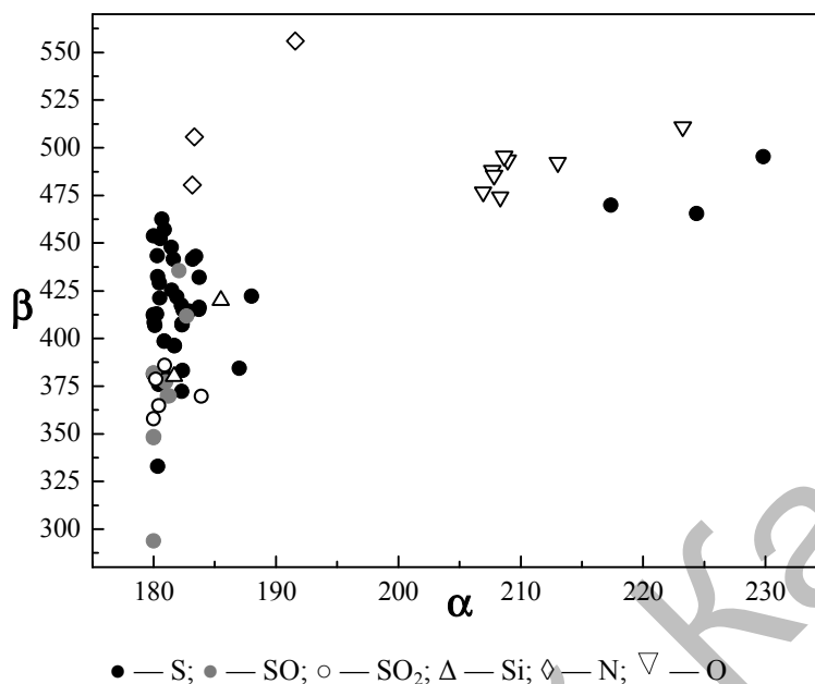
Figure 20. The \alpha - \beta plot of all 1,3-alternate heteroatom-bridged calix[4]arenes divided according to the type of the bridge
