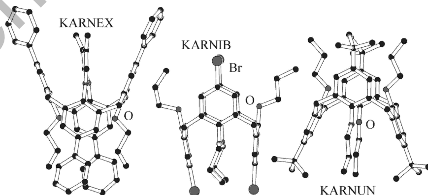
Figure II-17: Structures KARNEX, KARNIB and KARNUN [10]
