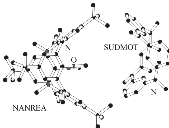
Figure II-24. Structures NANREA, SUDMOT [10]
