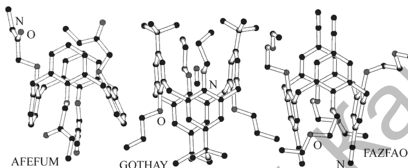
Figure II-16. Structures AFEFUM ( \beta \sim 425^\circ ), GOTHAY ( \beta \sim 370^\circ ) and FAZFAO ( \beta \sim 320^\circ ) [10] demonstrating effects of a filled and empty 'cavity' on the geometry of the calix[4]arene base frame
