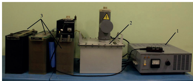
Fig. 1. An electric pulse plant. 1 – a control panel, 2 – a generator with a discharger, 3 – a protection unit with a capacitor
