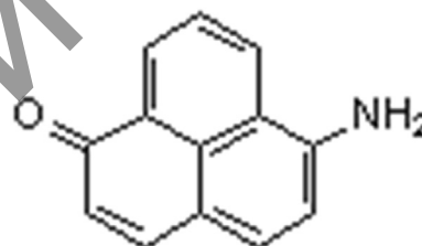
Fig. 3. The structural formula of 6-Amino-1H-phenalen-1-one (Ph160).
