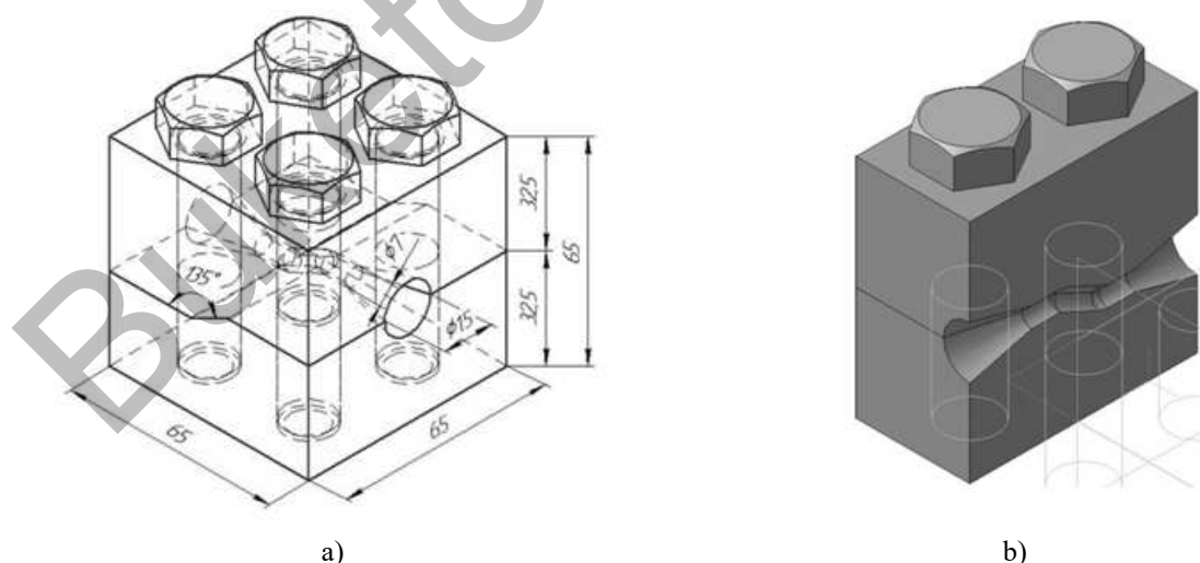
Fig.1. Matrix for equal-channel angular drawing: a) - matrix scheme, b) - 3D model
