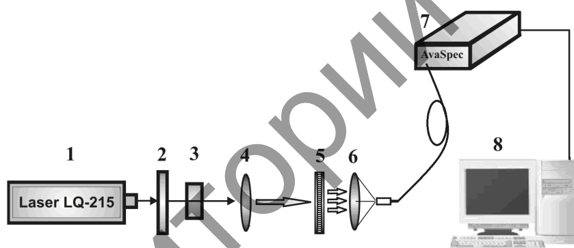
Fig. 1. Installation for investigating the characteristics of stimulated emission of thin films:. 1 – LQ 215; 2 – neutral density filters; 3 – diaphragm; 4.6 – lens; 5 – sample; 7 – AvaSpec-2048; 8 – computer
