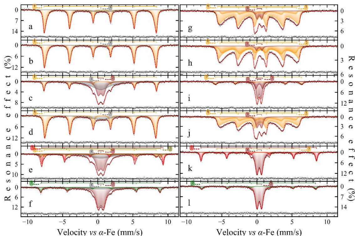
Figure 2. Mössbauer spectra of samples recorded at 78 K (a–f) and 296 K (g–l): A-N (a, g), A-C (b, h), U-N (c, i), U-C (d, j), H-N (e, k), and H-C (f, l). Subspectra are labeled in accordance with Table 3. Error bars for the experimental data points are shown; residuals obtained by subtracting the fitted model from the experimental spectra are displayed beneath each corresponding plot
