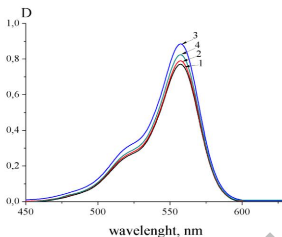
Fig.3. Influence of Au nanoparticles on the Rhodamin C absorption in ethanol: 1 – 0; 2 – 2 \cdot 10^{-6} mol/l; 3 – 5 \cdot 10^{-6} mol/l; 4 – 5 \cdot 10^{-5} mol/l.
