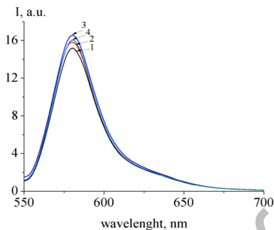
Fig.4. Effect of Au nanoparticles on Rhodamin C fluorescence in ethanol: 1 – 0; 2 – 2 \cdot 10^{-6} mol/l; 3 – 5 \cdot 10^{-6} mol/l; 4 – 5 \cdot 10^{-5} mol/l.
