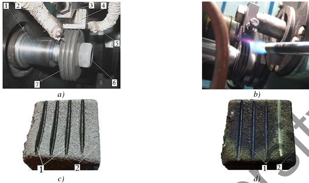
Fig. 1. Elements of methodological support for experimental studies: a) contact of the disk samples with the pad: 1 - lower shaft of the SMC-2 friction machine; 2 - thermocouple casing; 3 - holder; 4 - coated sample pad; 5 - thermocouple casing; 6 - fixing nut; 7 - sample disk with ridges; b) contact of the sample disk with the pad in a burning gas mixture; c) the surface of the coating formed by the gas-flame method; d) the surface of the coating formed by the gas-flame method after temperature loading in a burning gas mixture: 1 - cut-in tracks; 2 – coating.
