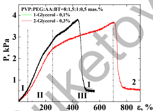
Figure 8. Deformation curves of hybrid composite materials P[AA-PVP-PEG]{BT} at different glycerol content
