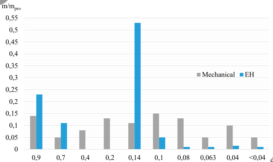
Fig. 5. Histogram of particle distribution during mechanical and electrohydroimpulse processing of Shubarkol coal
