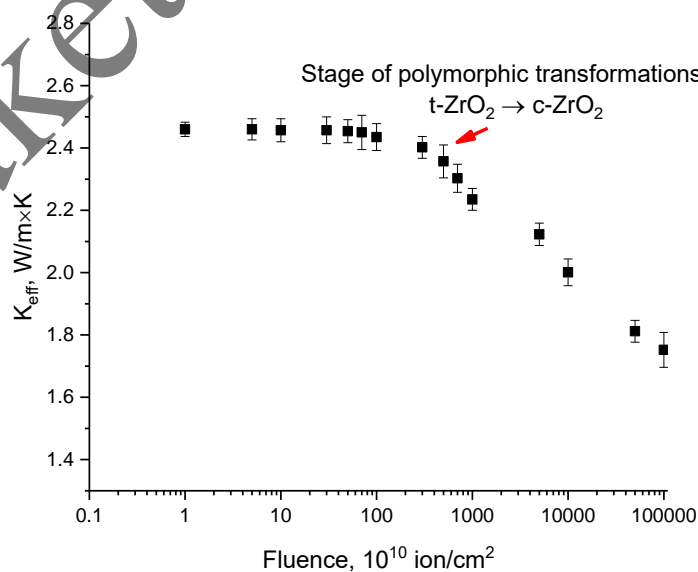
Fig.3. Results of the change in the thermal conductivity coefficient from the irradiation fluence
