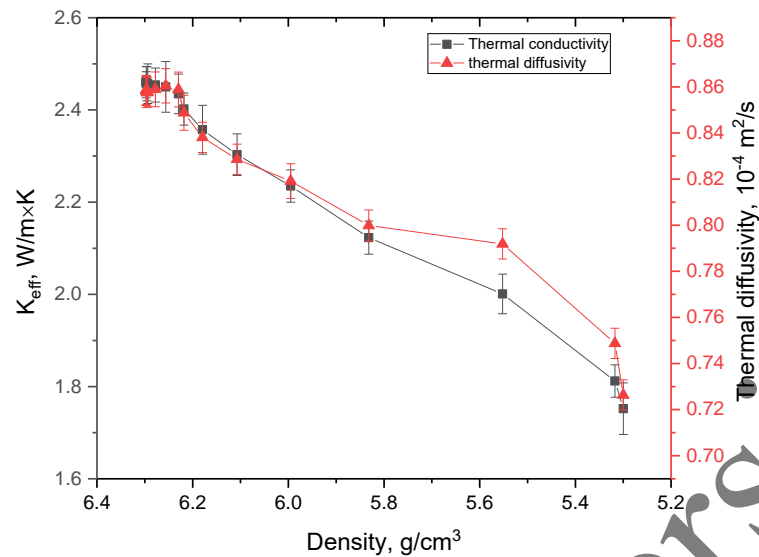
Fig.5. Dependence of changes in thermophysical parameters on the density of ceramics
