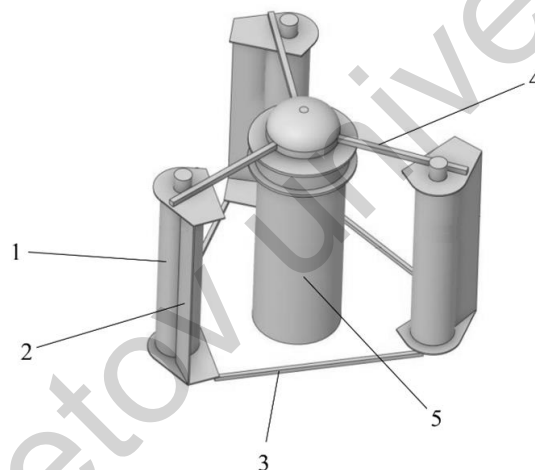
Fig. 1. Wind turbine with combined blades: 1 – cylinder rotating around its axis; 2 – fixed blade; 3, 4 – retaining rods; 5 – support of the wind turbine
