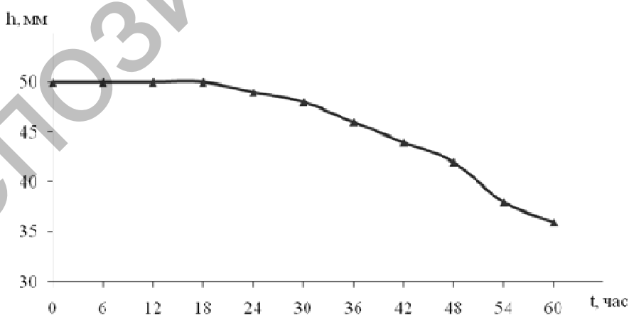
Figure 4. Dependence of the height of the dispersed phase layer on the time of the suspension with the addition of fuel oil M-100
