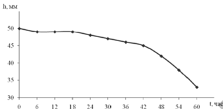
Figure 5. Dependence of the height of the dispersed phase layer on the time of the suspension with the addition of lignosulfonate
