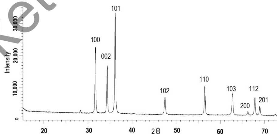
Figure 2. X-ray diffraction (XRD) pattern of the synthesized biogenic ZnO NPs.
