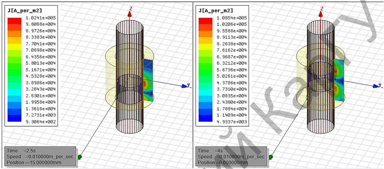
a) at 2,5 second of skip motion; b) at the 4th second of skip motion Fig.1. Calculation results of the Lorentz force of initial model
