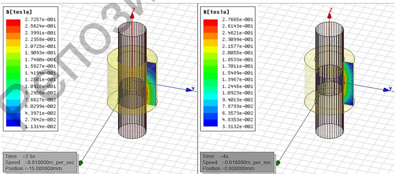
a) at 2.5 second of skip motion; b) at the 4th second of skip motion Fig.2. Calculation results of magnetic induction B of initial models
