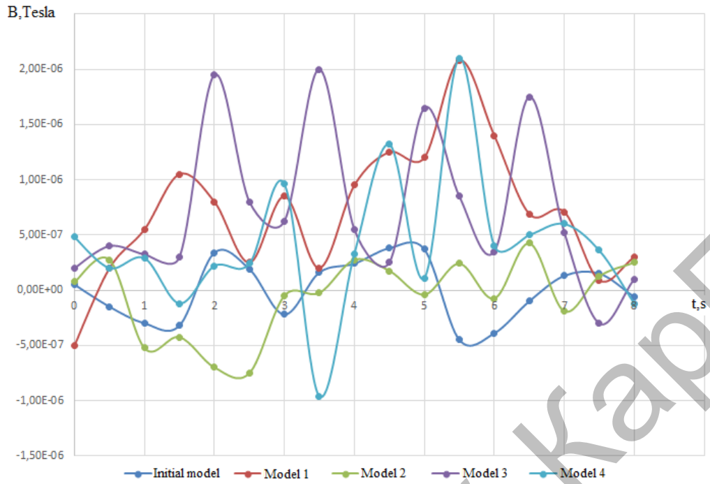
Fig.8. Family of dependences of magnetic field induction on time
