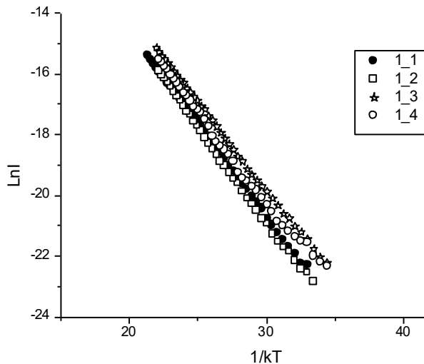
Fig.3. The temperature dependence of conductivity current for samples without ZrO_2
