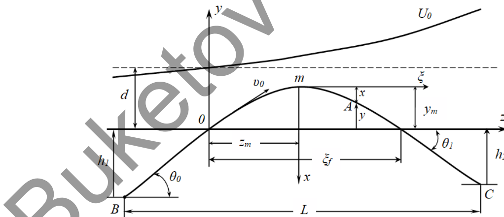
Fig.2. The electrostatic mirror based on non-uniform field.
