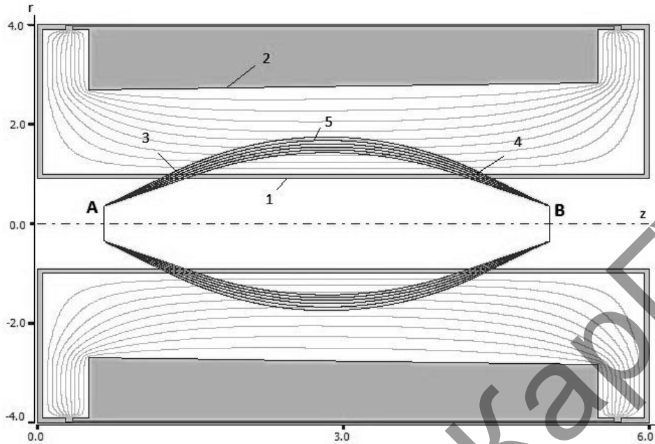
1 – the inner grounded cylindrical electrode, 2 – the outer deflecting electrode, 3 and 4 - entrance and exit slits, A - thin ring source, B - ring image, 5- charged particles beam
