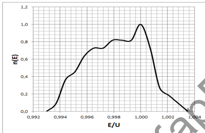
Fig. 6. The instrumental function of the quadrupole-cylindrical energy analyzer with A=0.01
