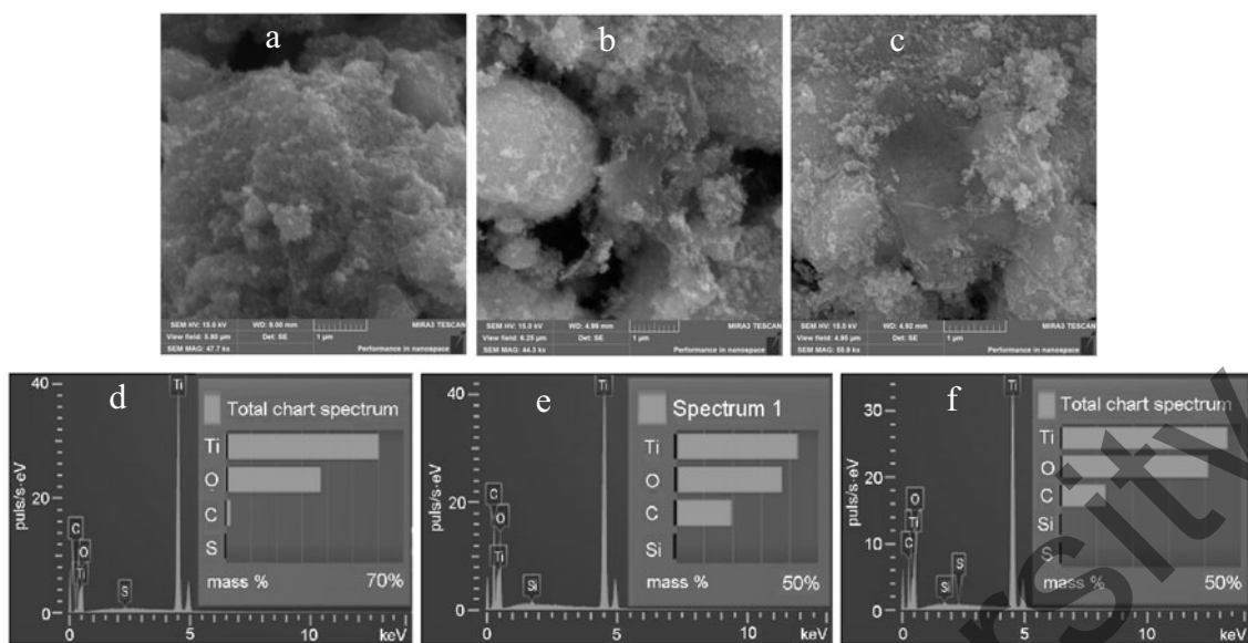
Fig. 1. SEM images (a-c) and energy-dispersive X-ray diffraction (d-f) of nanocomposite material: a, d) \text{TiO}_2 -rGO/1%, b, e) \text{TiO}_2 -rGO/5%, and c, f) \text{TiO}_2 -rGO/10%.
