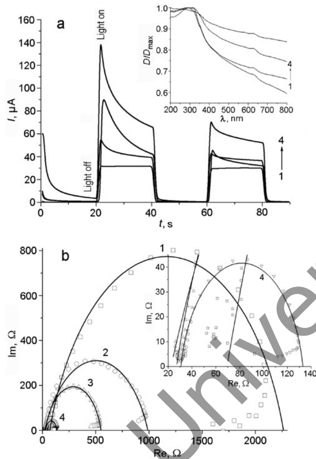
Fig. 3. Transitional characteristics of the photocurrent of samples (a) (insert gives the absorption spectra) and Nyquist plot of the impedance spectrum (b): 1) \text{TiO}_2 , 2) \text{TiO}_2 -rGO/1%, 3) \text{TiO}_2 -rGO/5%, and 4) \text{TiO}_2 -rGO/10% (insert gives Nyquist plot for the impedance spectrum for \text{TiO}_2 -rGO/10% in an enlarged scale).
