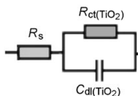
Fig. 4. Equivalent electrical scheme of the electrochemical cell.
