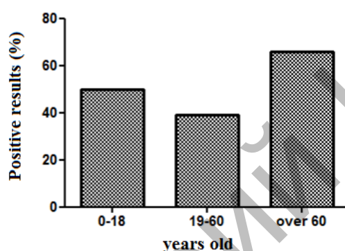
Figure 1. Positive results of Helicobacter pylori determination in different age categories
