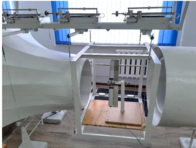
Figure 1. An experimental sample of a two-bladed layout
