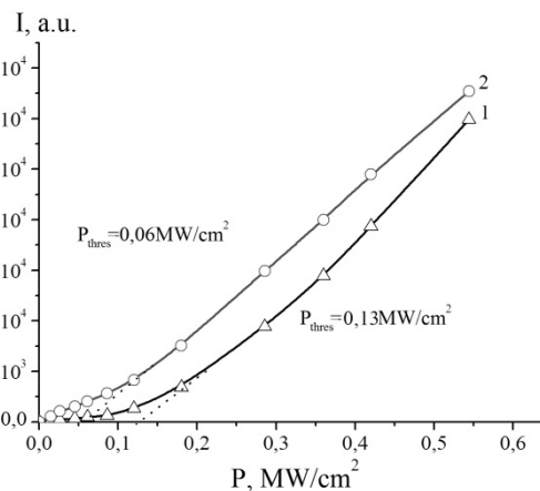
1 — pure dye; 2 — Ph160 with 10^{-4} mol/l Au nanoparticles
