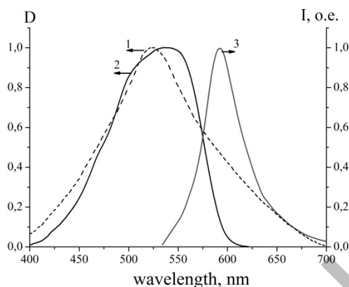
Figure 3. Relative location of the absorption spectra of Au nanoparticles (1), Ph160 (2) and dye fluorescence (3)
