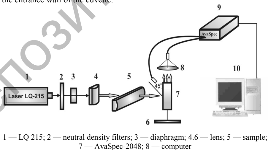
Figure 2. Diagram of an experimental setup for investigating the generation characteristics of molecular systems
