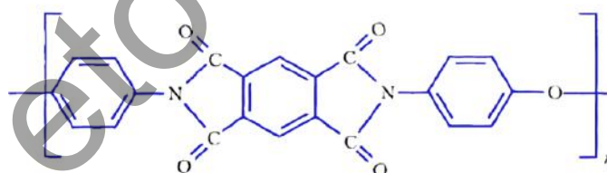
Fig.1. Structural Unit of a Polyimide Macromolecule [29]
