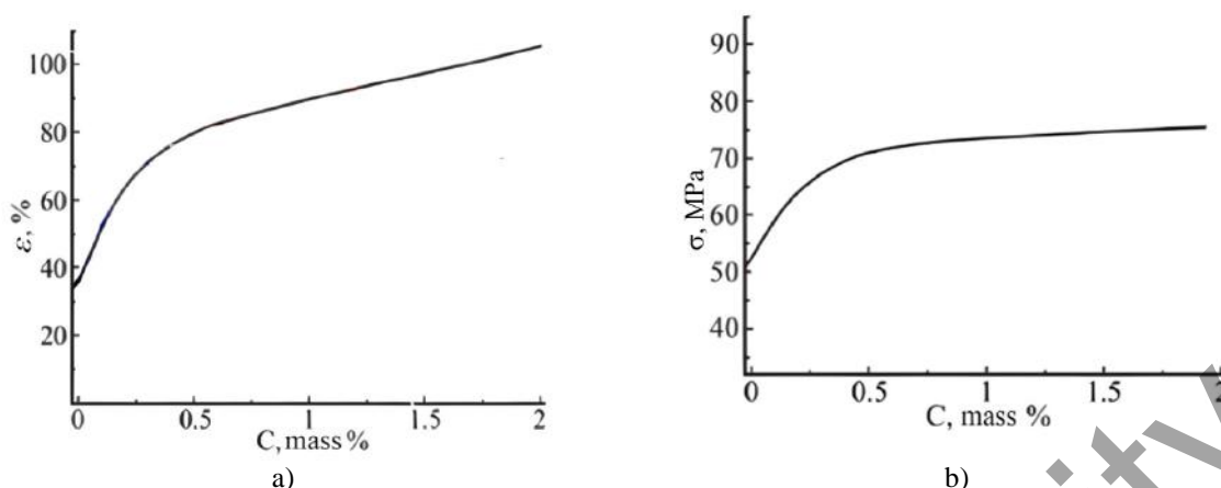
Fig.4. a) Effect of PT filler concentration (C) on elongation at break ( \varepsilon ) of polyimide composite materials at room temperature. b) Effect of PT filler concentration (C) on tensile strength ( \sigma ) of polyimide composite materials at room temperature.
