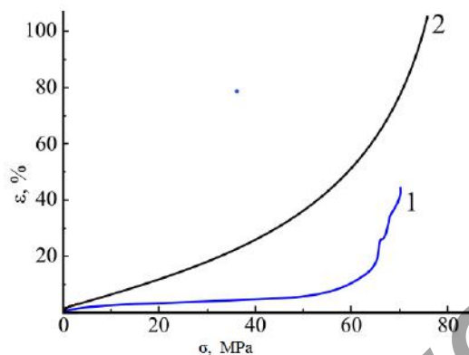
Fig. 3. The dependence of relative elongation ( \varepsilon ) on mechanical load ( \sigma ) for pure polyimide film (curve 1) and polyimide composites with PT filler (curve 2), measured at room temperature.
