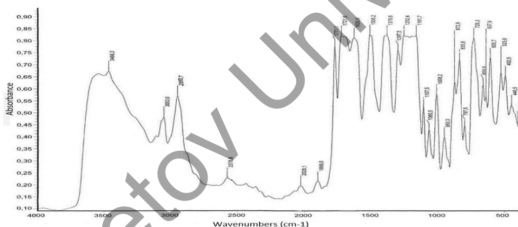
Fig.7. IR spectrum of polyimide film after film rupture
