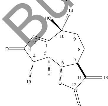
Figure 1. Structural formula of molecule 3-oxo-10 \beta -hydroxy-5,7 \alpha (H),6 \beta (H)-guaia-1,11(13)-diene-6,12-olide ( 1 )
