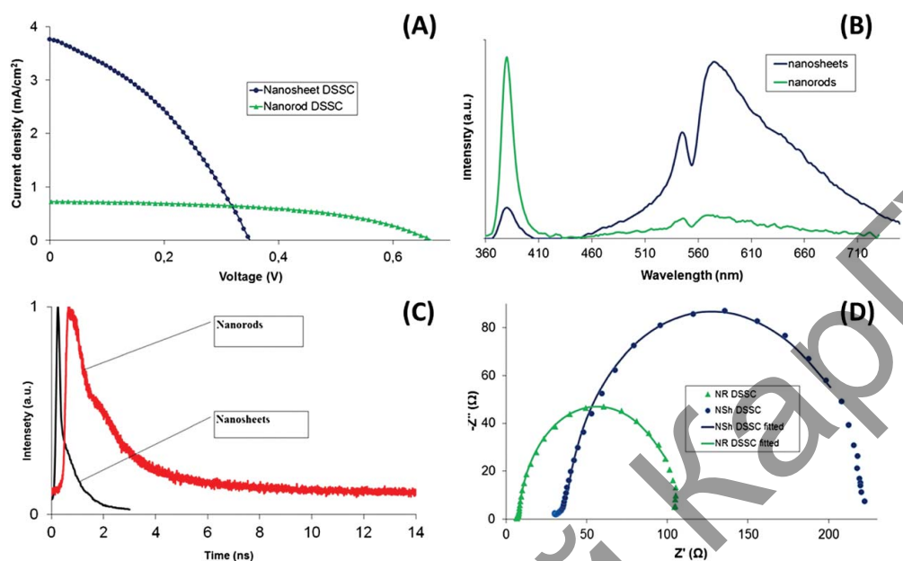
Figure 4. (Colour online). (A) Current-voltage characteristic of DSSCs based on the ZnO nanorod (green line) and nanosheet (blue line) arrays. (B) The normalised PL spectra of nanosheet (blue line) and nanorod (green line) arrays of ZnO. (C) Decay kinetics of the edge luminescence band (ELB) of the ZnO nanorods (red line) and nanosheets (blue line). (D) Nyquist plots of DSSCs performed under illumination at the applied bias of V_{OC} . The solid lines are the fitting results from the equivalent circuit model of ZnO DSSCs.
