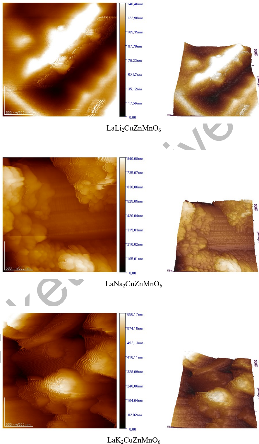
Fig. 2. Atomic-force microscopic image and 3D surfaces
