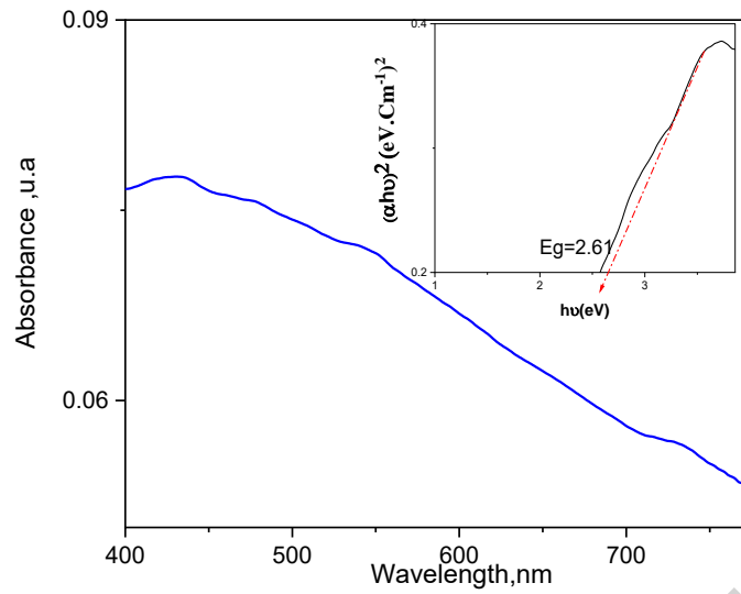
Figure 4. Tauc plots of ZnMn 2 O 4 nanoparticles
