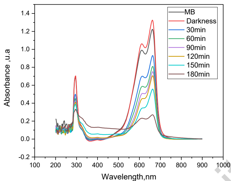
Figure 10. Photocatalytic degradation of Methylene Blue (MB) by 3 % Cu-doped ZnMn_2O_4 , synthesized with an MB concentration of 10 mg/L and a 1 % Cu-doped ZnMn_2O_4 concentration of 0.1 g/L
