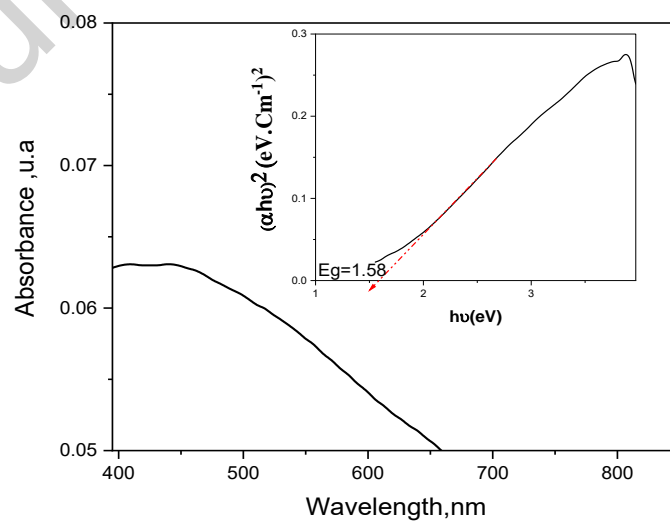
Figure 6. Tauc plots of ZnMn 2 O 4 NPs doped with 3% Cu
