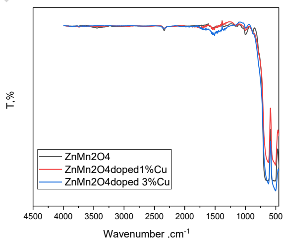
Figure 1. FTIR absorption spectra of all Cu-doped \text{ZnMn}_2\text{O}_4 compounds
